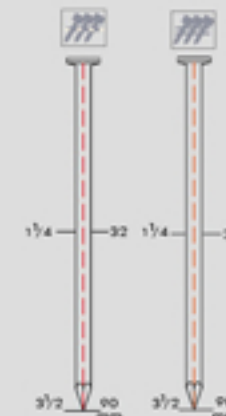
PCN-790H CONCRETE COIL NAILER
