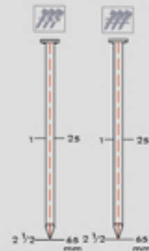
PCN-565S PRO-COIL NAILER
