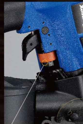
ADJUSTABLE WORK CONTACTING ELEMENT Depth of drive adjustment by wheel. (U.S. PATENT 6866177)
