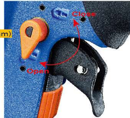
Safety Trigger Lock Level
