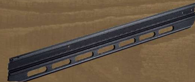
EXTENDED MAGAZINE FOR AUTOMATIC PRE-NAIL MACHINE (4 STRIPS)
